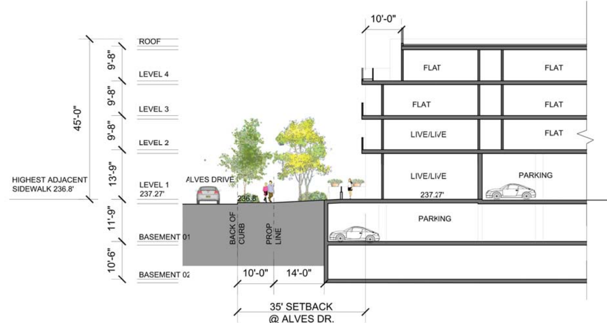
3 SIDEWALK SECTION
