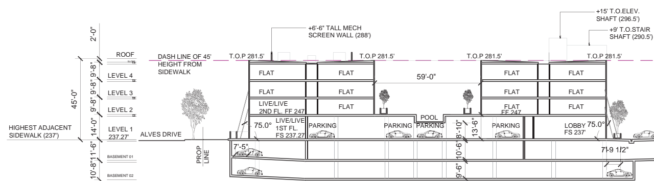
13 APARTMENT BUILDING B SECTION
