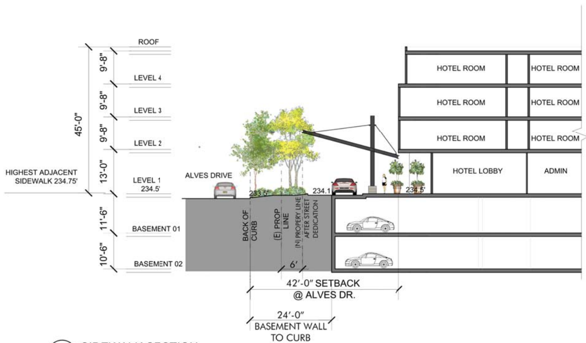
2 SIDEWALK SECTION
