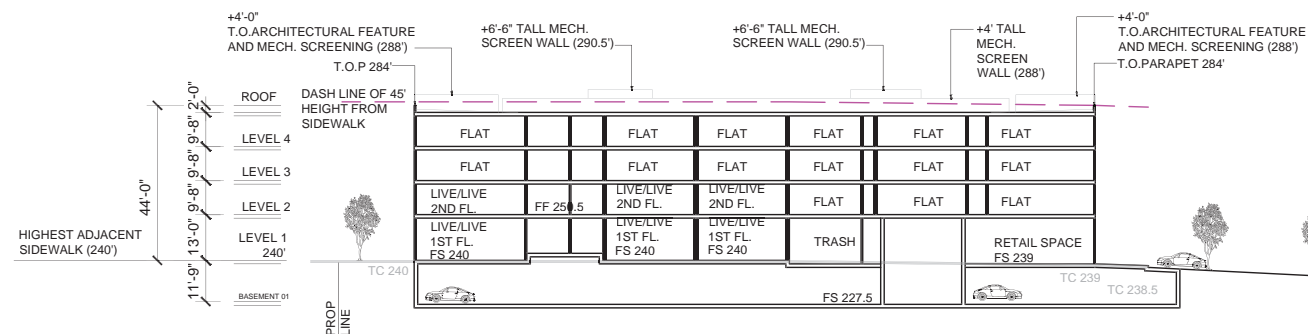
11 APARTMENT BUILDING C SECTION
