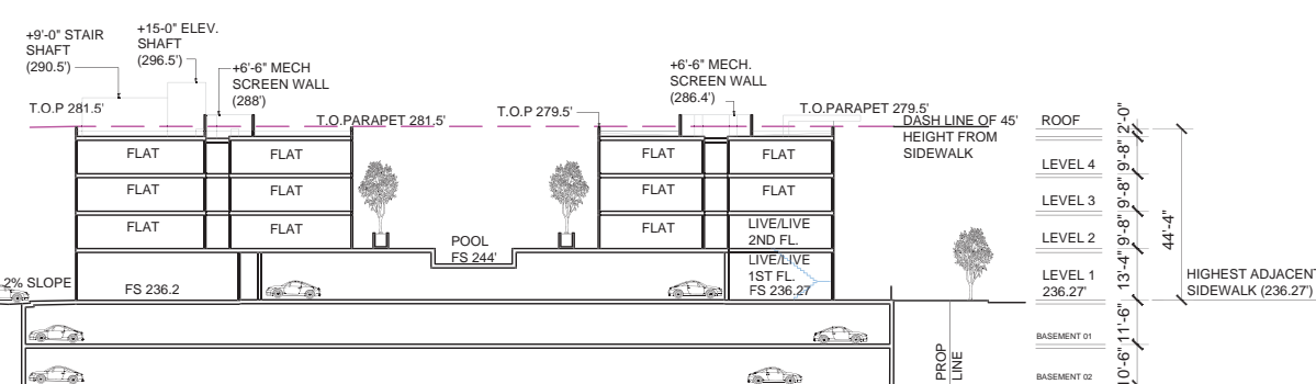
12 APARTMENT BUILDING B SECTION
