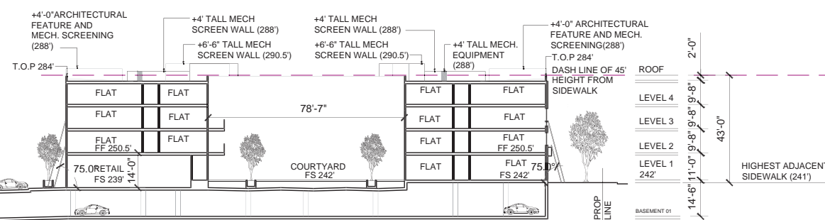
14 APARTMENT BUILDING C SECTION
