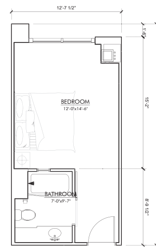
HOTEL ROOM E2 (2) BED UNIT FLOOR PLAN GROSS AREA: 305 SQFT NET AREA: 262 SQFT
