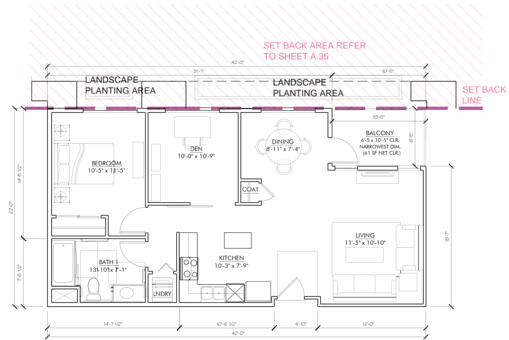
UNIT K1 (1) BED + DEN UNIT PLAN GROSS AREA: 853 SQFT NET AREA: 787 SQFT BALCONY: 61 SQFT
