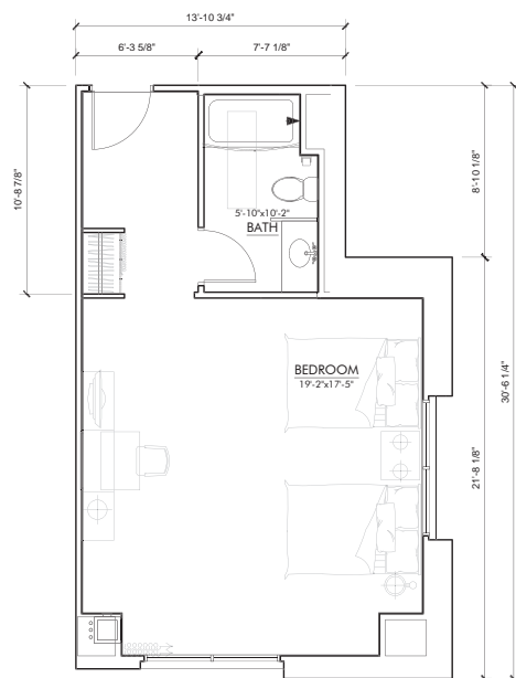
HOTEL ROOM B2 (2) BED UNIT FLOOR PLAN GROSS AREA: 528 SQFT NET AREA: 435 SQFT
