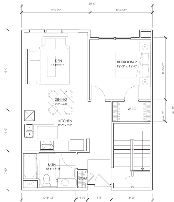
UNIT TW3-2 (SECOND LEVEL) (2) BED UNIT PLAN
