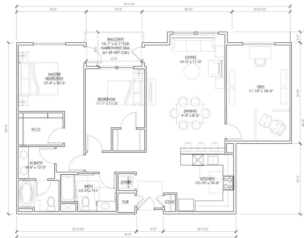
UNIT R1 (2) BED + DEN UNIT PLAN GROSS AREA: 1,475 SQFT NET AREA: 1,393 SQFT BALCONY: 61 SQFT
