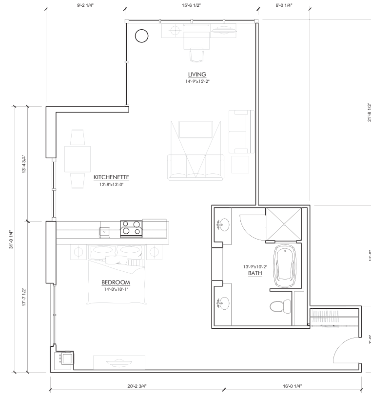
HOTEL ROOM G1 KING ROOM SUITE UNIT GROSS AREA: 1079 SQFT NET AREA: 981 SQFT
