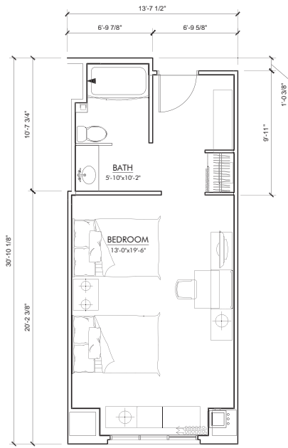
HOTEL ROOM A13 & A15 (SIM) (2) BED UNIT FLOOR PLAN GROSS AREA: 413 SQFT NET AREA: 359 SQFT
