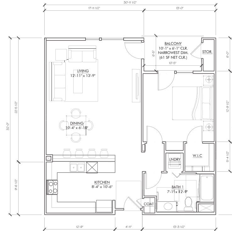
UNIT A6 (1) BED UNIT PLAN GROSS AREA: 924 SQFT NET AREA: 852 SQFT BALCONY: 61 SQFT
