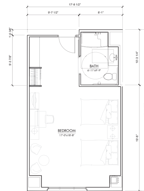
HOTEL ROOM-C1 (2) BED UNIT FLOOR PLAN GROSS AREA: 514 SQFT NET AREA: 458 SQFT
