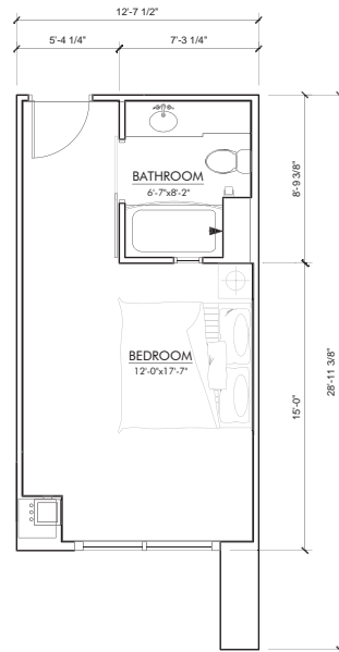
HOTEL ROOM E1 KING BED UNIT FLOOR PLAN GROSS AREA: 310 SQFT NET AREA: 268 SQFT
