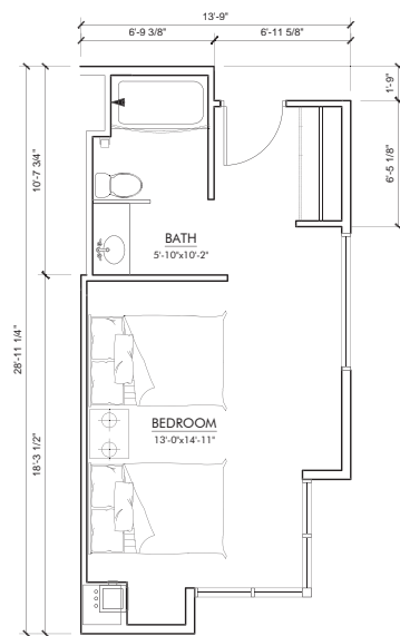
HOTEL ROOM A4 (2) BED UNIT FLOOR PLAN (Typ. 4th Floor Plan) GROSS AREA: 358 SQFT NET AREA: 311 SQFT
