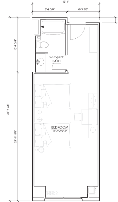
HOTEL ROOM B6 (2) BED UNIT FLOOR PLAN GROSS AREA: 459 SQFT NET AREA: 404 SQFT
