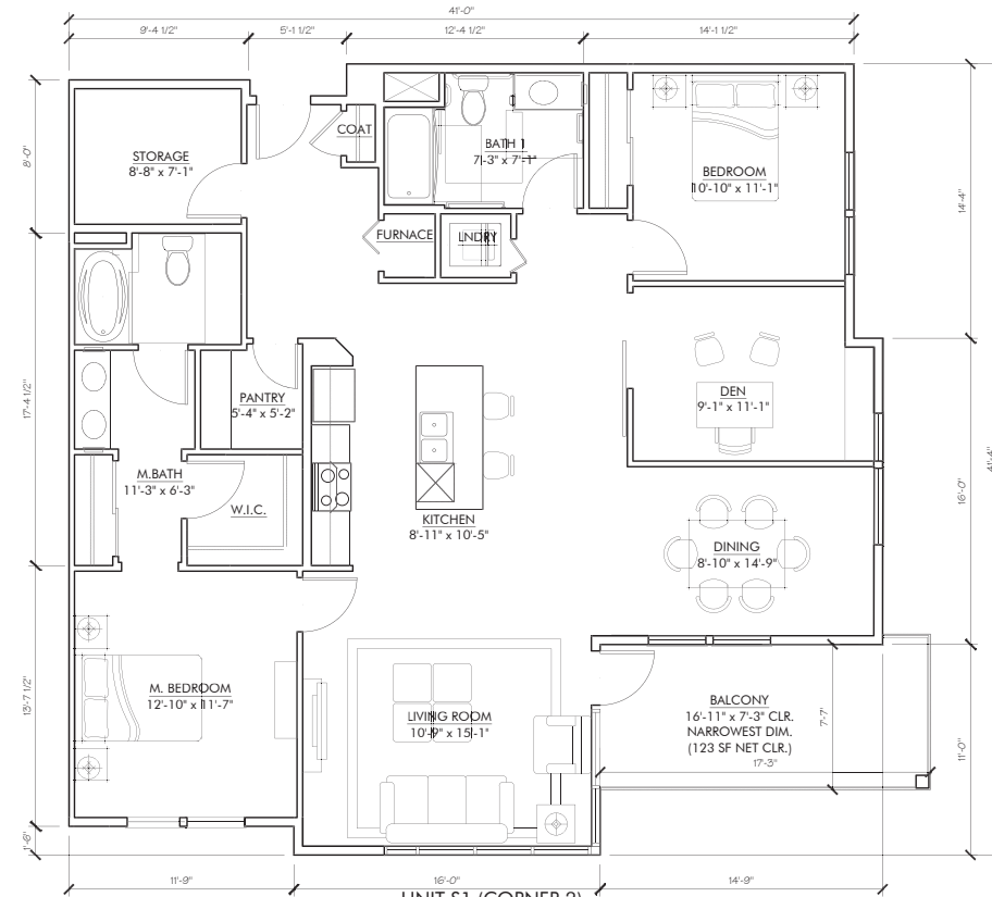
UNIT S1 (CORNER 2) (2) BED + DEN UNIT PLAN GROSS AREA: 1,539 SQFT NET AREA: 1,452 SQFT BALCONY: 123 SQFT
