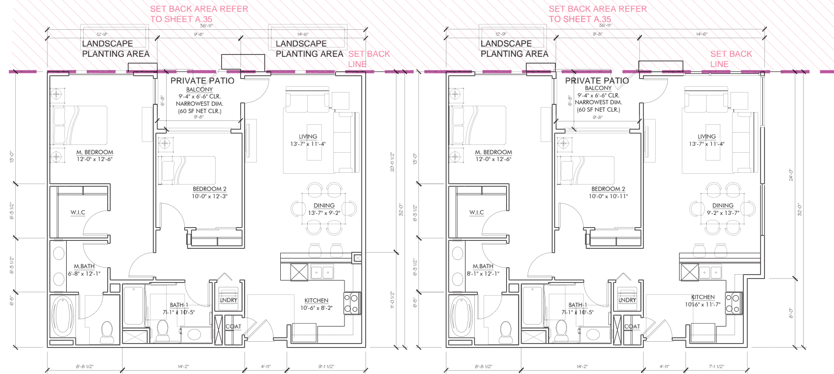
UNIT G2 - CORNER (2) BED UNIT PLAN GROSS AREA: 1097 SQFT NET AREA: 1013 SQFT BALCONY: 60 SQFT
