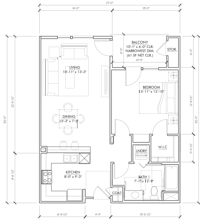
UNIT A1 (1) BED UNIT PLAN GROSS AREA: 797 SQFT NET AREA: 728 SQFT BALCONY: 61 SQFT
