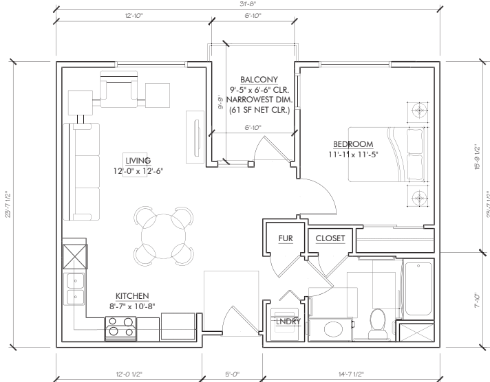
UNIT C1 (1) BED UNIT PLAN GROSS AREA: 687 SQFT NET AREA: 617 SQFT BALCONY: 61 SQFT
