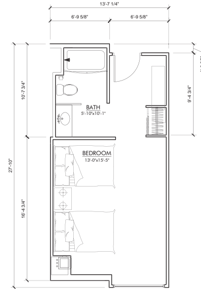
HOTEL ROOM A2-a (2) BED UNIT FLOOR PLAN (Typ. 4th Floor Plan) GROSS AREA: 365 SQFT NET AREA: 323 SQFT
