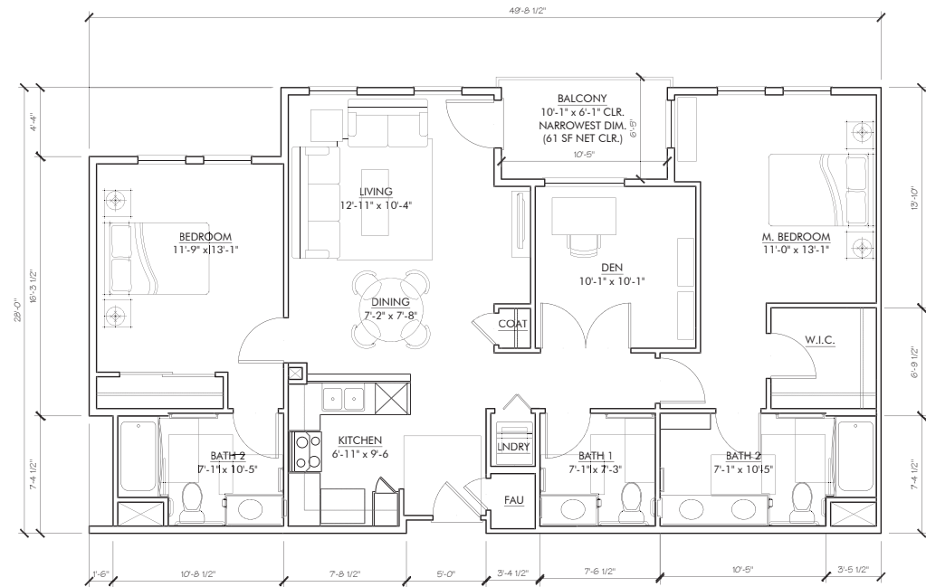
UNIT H2 (2) BED + DEN UNIT PLAN GROSS AREA: 1264 SQFT NET AREA: 1175 SQFT BALCONY: 61 SQFT
