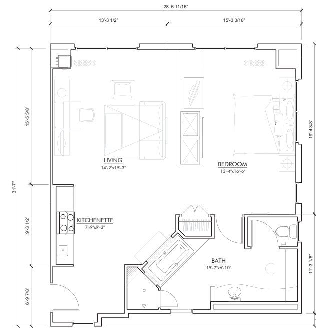
HOTEL ROOM F1 SUITE UNIT FLOOR PLAN GROSS AREA: 885 SQFT NET AREA: 802 SQFT
