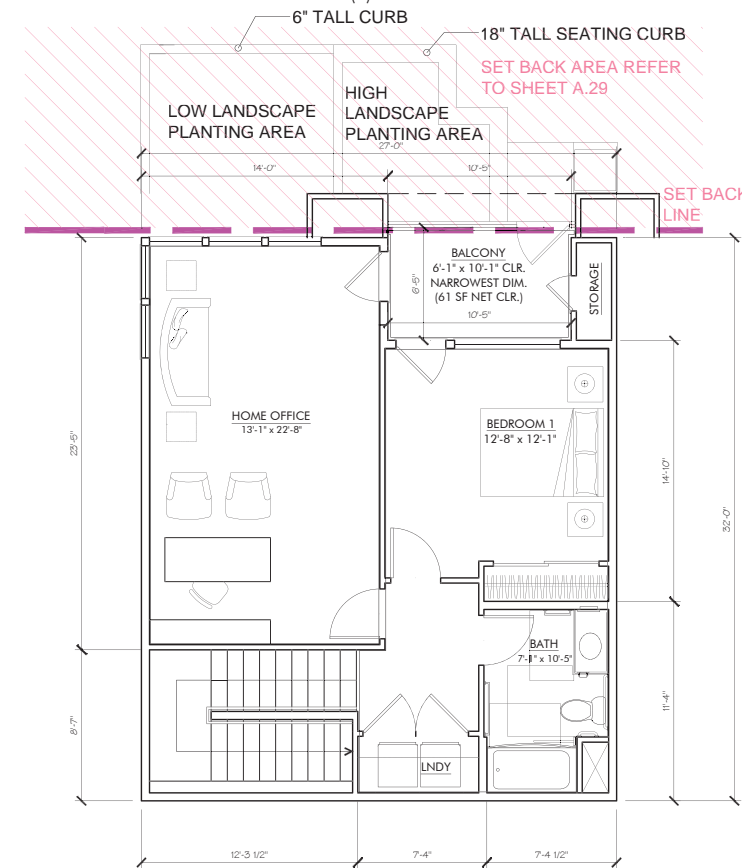
UNIT TW2-1 (FIRST LEVEL) REVERSE (2) BED UNIT PLAN
