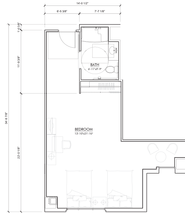
HOTEL ROOM-C4 (2) BED UNIT FLOOR PLAN GROSS AREA: 601 SQFT NET AREA: 528 SQFT
