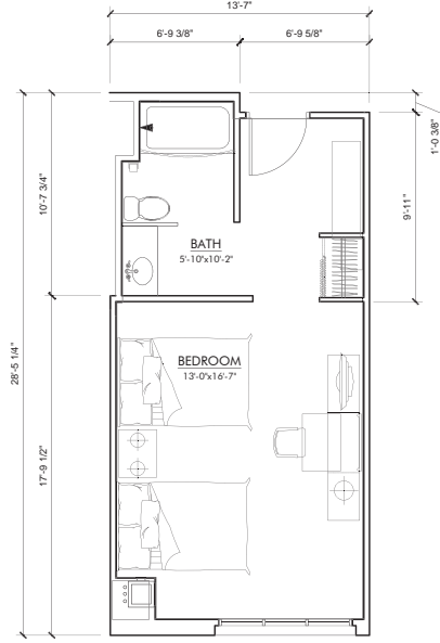
HOTEL ROOM A14 & A12 (SIM) (2) BED UNIT FLOOR PLAN (Typ. 4th Floor Plan) GROSS AREA: 379 SQFT NET AREA: 332 SQFT
