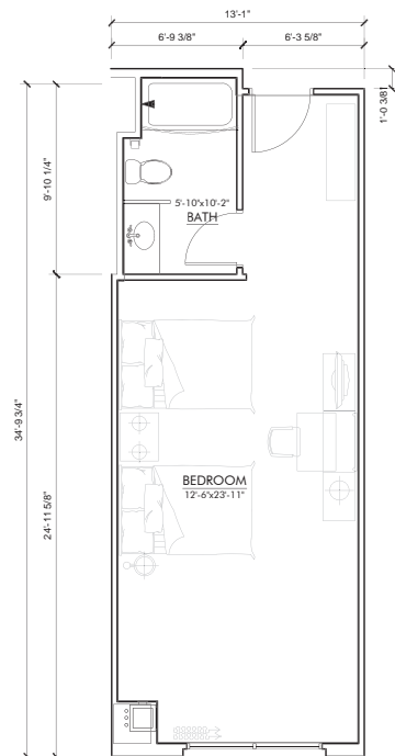
HOTEL ROOM B3 (2) BED UNIT FLOOR PLAN GROSS AREA: 459 SQFT NET AREA: 409 SQFT
