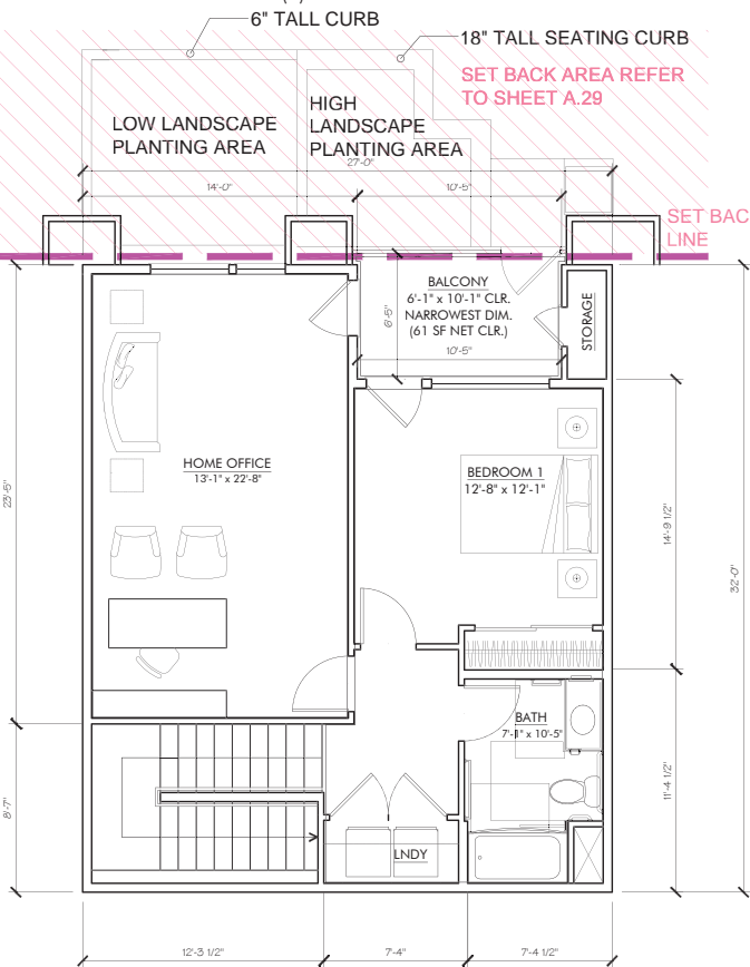
UNIT TW1-1 (FIRST LEVEL) (2) BED UNIT PLAN
