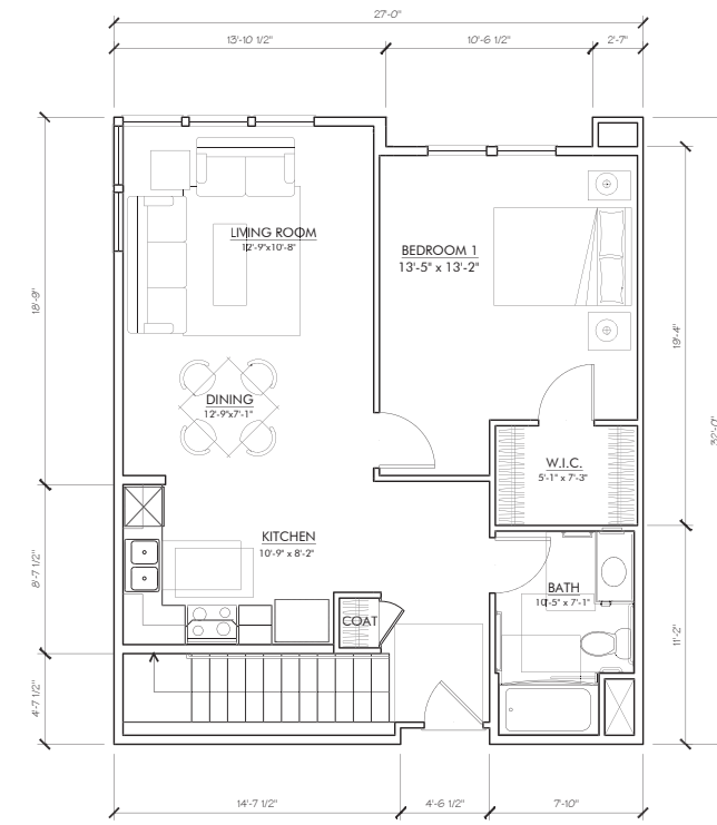
UNIT TW2-2 (SECOND LEVEL) (2) BED UNIT PLAN
