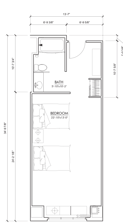
HOTEL ROOM A1 (2) BED UNIT FLOOR PLAN GROSS AREA: 466 SQFT NET AREA: 411 SQFT
