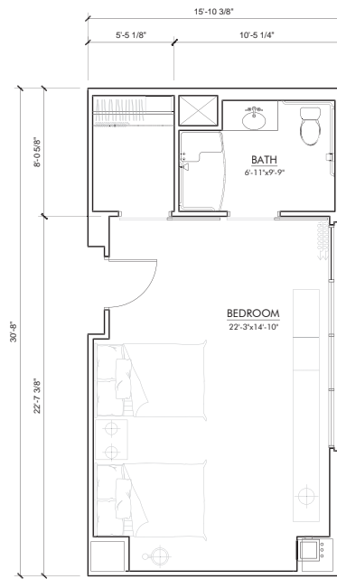
HOTEL ROOM D1 (2) BED UNIT FLOOR PLAN GROSS AREA: 481 SQFT NET AREA: 416 SQFT
