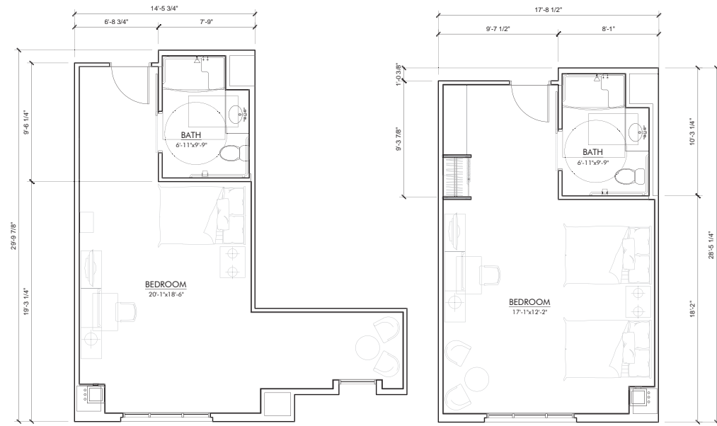
HOTEL ROOM-C2 (2) BED UNIT FLOOR PLAN GROSS AREA: 513 SQFT NET AREA: 448 SQFT
