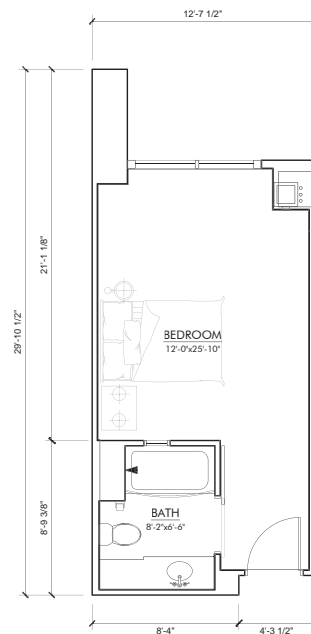
HOTEL ROOM H1 1 BED UNIT FLOOR PLAN GROSS AREA: 317 SQFT NET AREA: 271 SQFT
