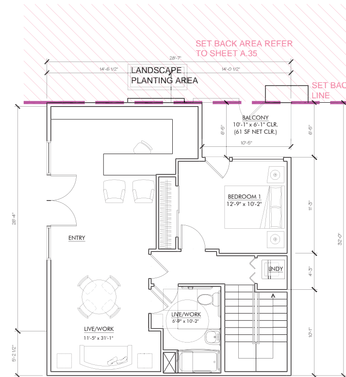
UNIT TW4-1 (FIRST LEVEL) (2) BED UNIT PLAN
