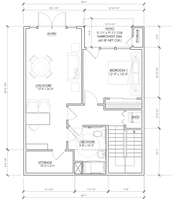
UNIT TW3-1 (FIRST LEVEL) (2) BED UNIT PLAN
