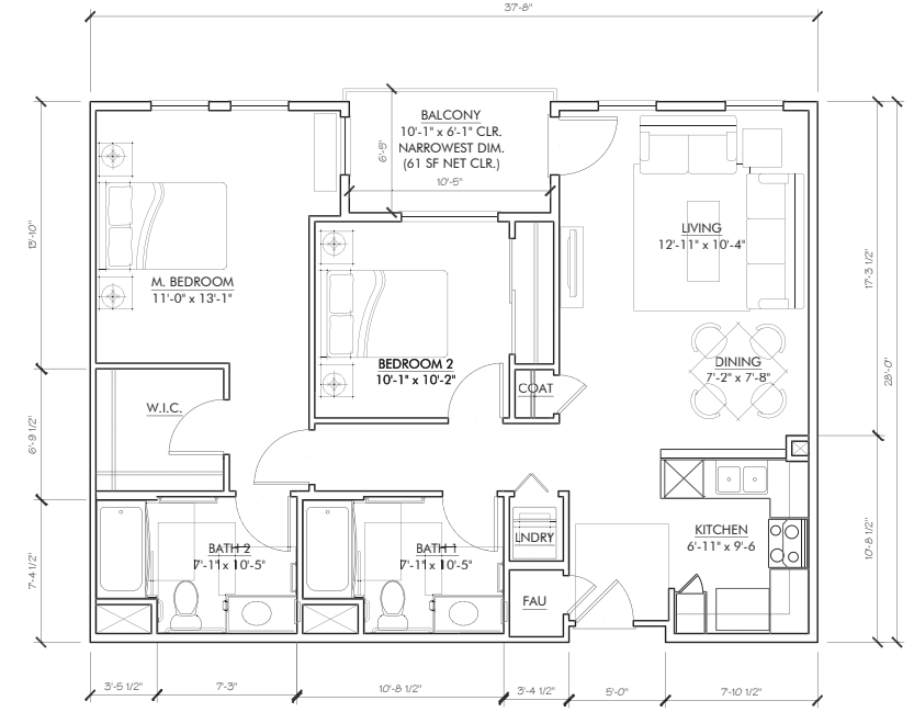
UNIT H1 (2) BED UNIT PLAN GROSS AREA: 991 SQFT NET AREA: 910 SQFT BALCONY: 61 SQFT
