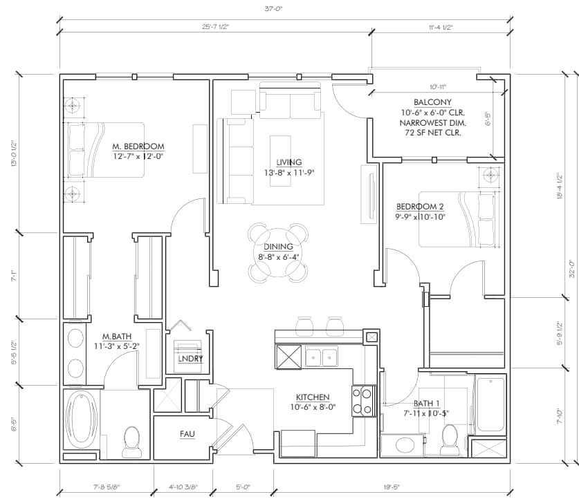
UNIT D2 (2) BED UNIT PLAN GROSS AREA: 1103 SQFT NET AREA: 1034 SQFT BALCONY: 72 SQFT
