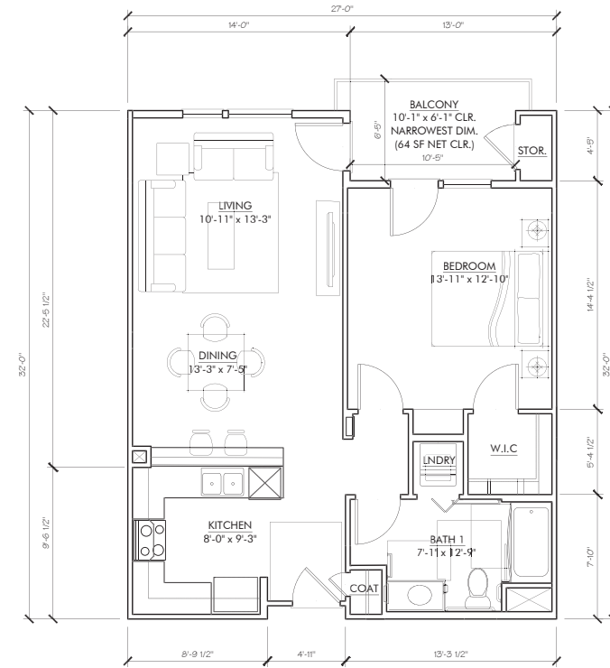
UNIT A3 (1) BED UNIT PLAN GROSS AREA: 814 SQFT NET AREA: 749 SQFT BALCONY: 64 SQFT
