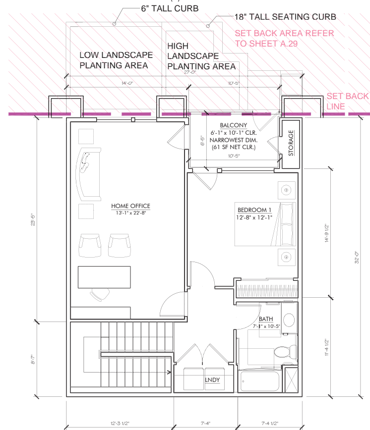
UNIT TW1-1 (FIRST LEVEL) (2) BED UNIT PLAN
