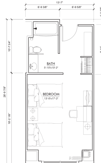
HOTEL ROOM A8 (2) BED UNIT FLOOR PLAN GROSS AREA: 384 SQFT NET AREA: 334 SQFT
