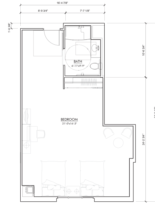
HOTEL ROOM-C5 (2) BED UNIT FLOOR PLAN GROSS AREA: 645 SQFT NET AREA: 576 SQFT
