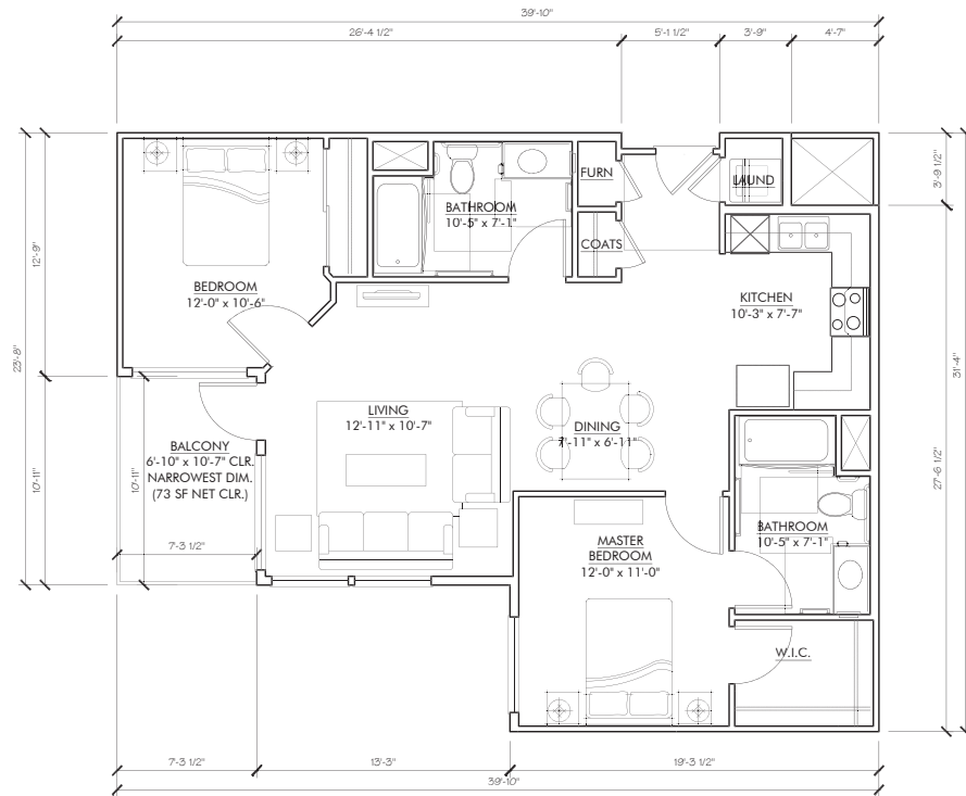
UNIT J1 (2) BED UNIT PLAN GROSS AREA: 1007 SQFT NET AREA: 914 SQFT BALCONY: 73 SQFT
