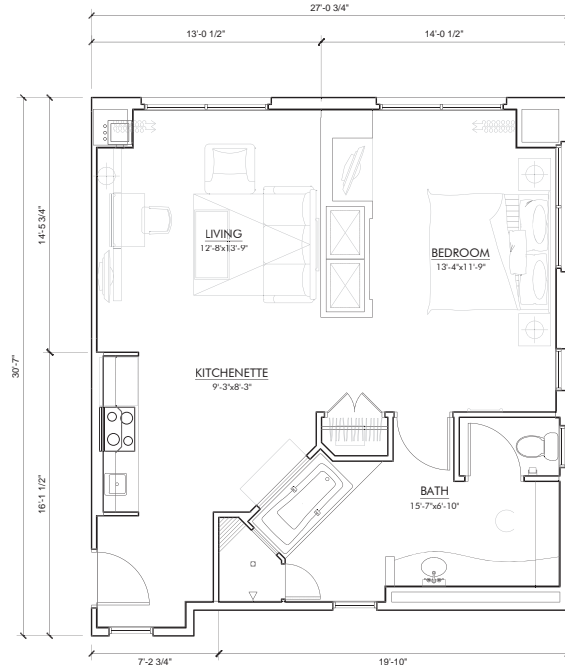
HOTEL ROOM F2 (1) BED SUITE FLOOR PLAN GROSS AREA: 797 SQFT NET AREA: 714 SQFT
