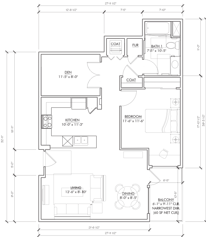
UNIT B1 (1) BED + DEN UNIT PLAN GROSS AREA: 925 SQFT NET AREA: 851 SQFT BALCONY: 60 SQFT
