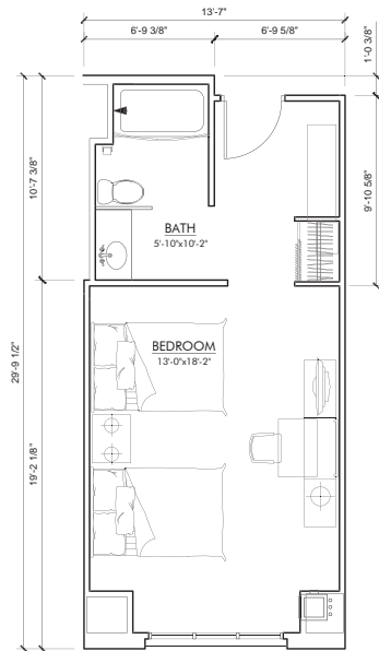
HOTEL ROOM A6 (2) BED UNIT FLOOR PLAN (Typ. 4th Floor Plan) GROSS AREA: 398 SQFT NET AREA: 345 SQFT
