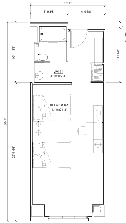
HOTEL ROOM A16 (2) BED UNIT FLOOR PLAN (Typ. 4th Floor Plan) GROSS AREA: 483 SQFT NET AREA: 424 SQFT
