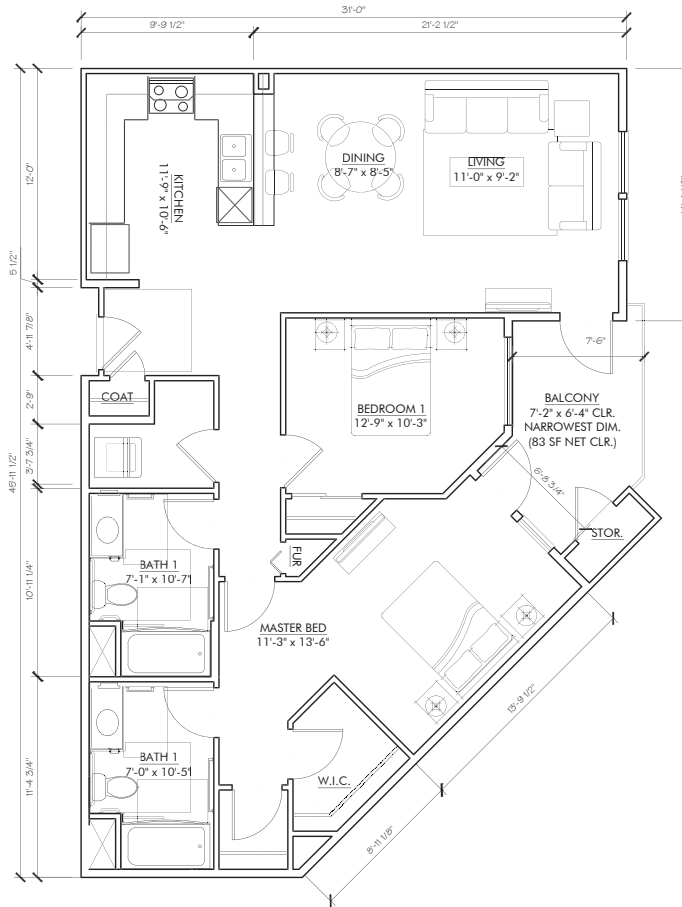
UNIT E1 (2) BED UNIT PLAN GROSS AREA: 1174 SQFT NET AREA: 1084 SQFT BALCONY: 83 SQFT
