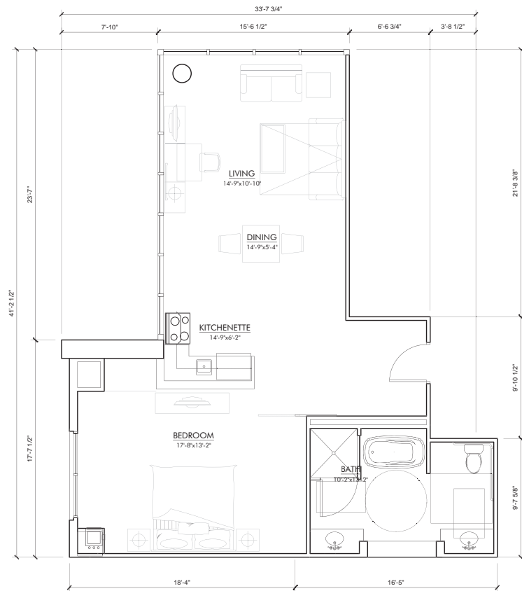
HOTEL ROOM G2 SUITE UNIT FLOOR PLAN GROSS AREA: 950 SQFT NET AREA: 864 SQFT
