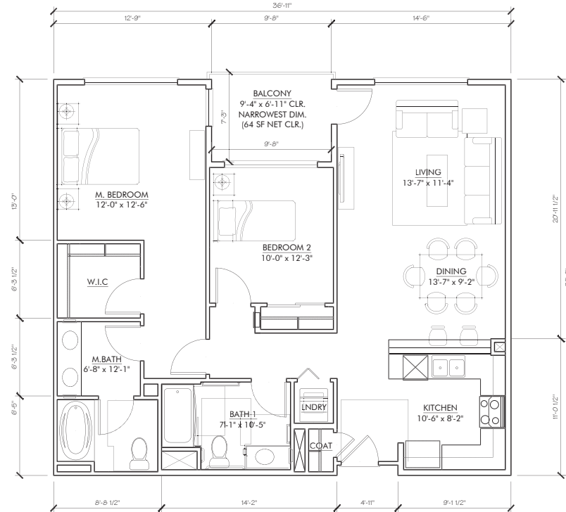
UNIT G3 (2) BED UNIT PLAN GROSS AREA: 1113 SQFT NET AREA: 1029 SQFT BALCONY: 64 SQFT
