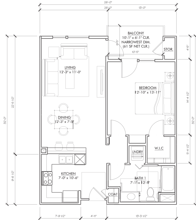
UNIT A4 (1) BED UNIT PLAN GROSS AREA: 782 SQFT NET AREA: 718 SQFT BALCONY: 61 SQFT
