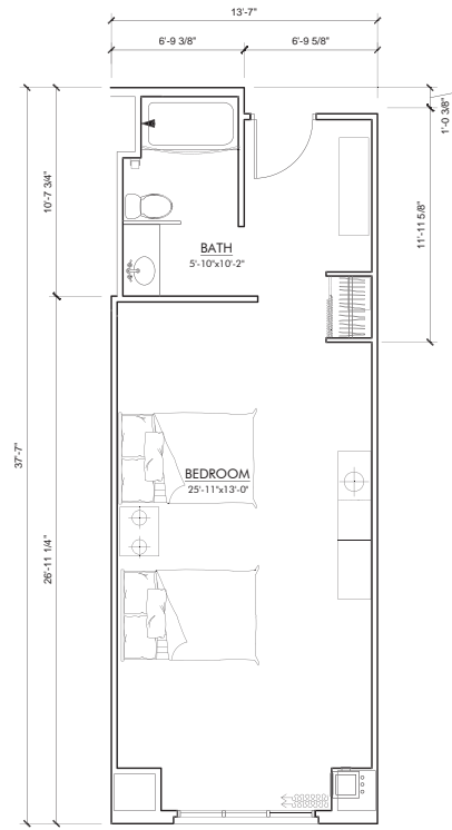
HOTEL ROOM A1-a (2) BED UNIT FLOOR PLAN GROSS AREA: 503 SQFT NET AREA: 445 SQFT
