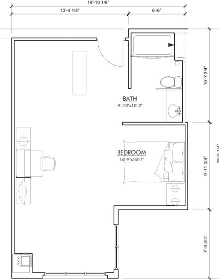
HOTEL ROOM A3 (2) BED UNIT FLOOR PLAN (Typ. 4th Floor Plan) GROSS AREA: 493 SQFT NET AREA: 445 SQFT
