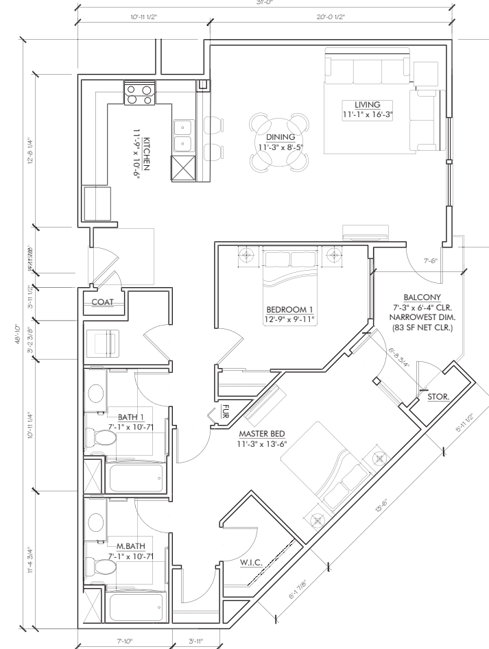
UNIT E2 (2) BED UNIT PLAN GROSS AREA: 1233 SQFT NET AREA: 1133 SQFT BALCONY: 83 SQFT
