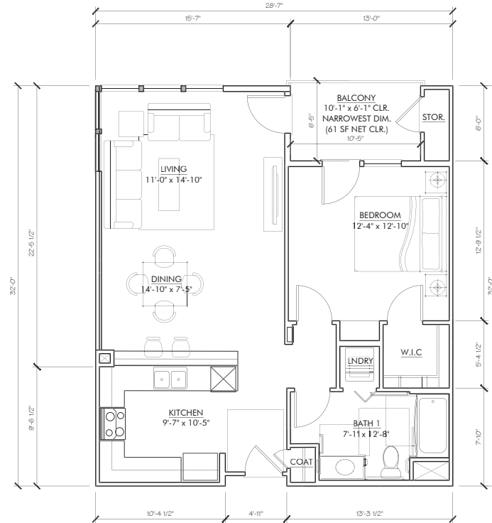
UNIT A5 (CORNER) (1) BED UNIT PLAN GROSS AREA: 848 SQFT NET AREA: 775 SQFT BALCONY: 61 SQFT
