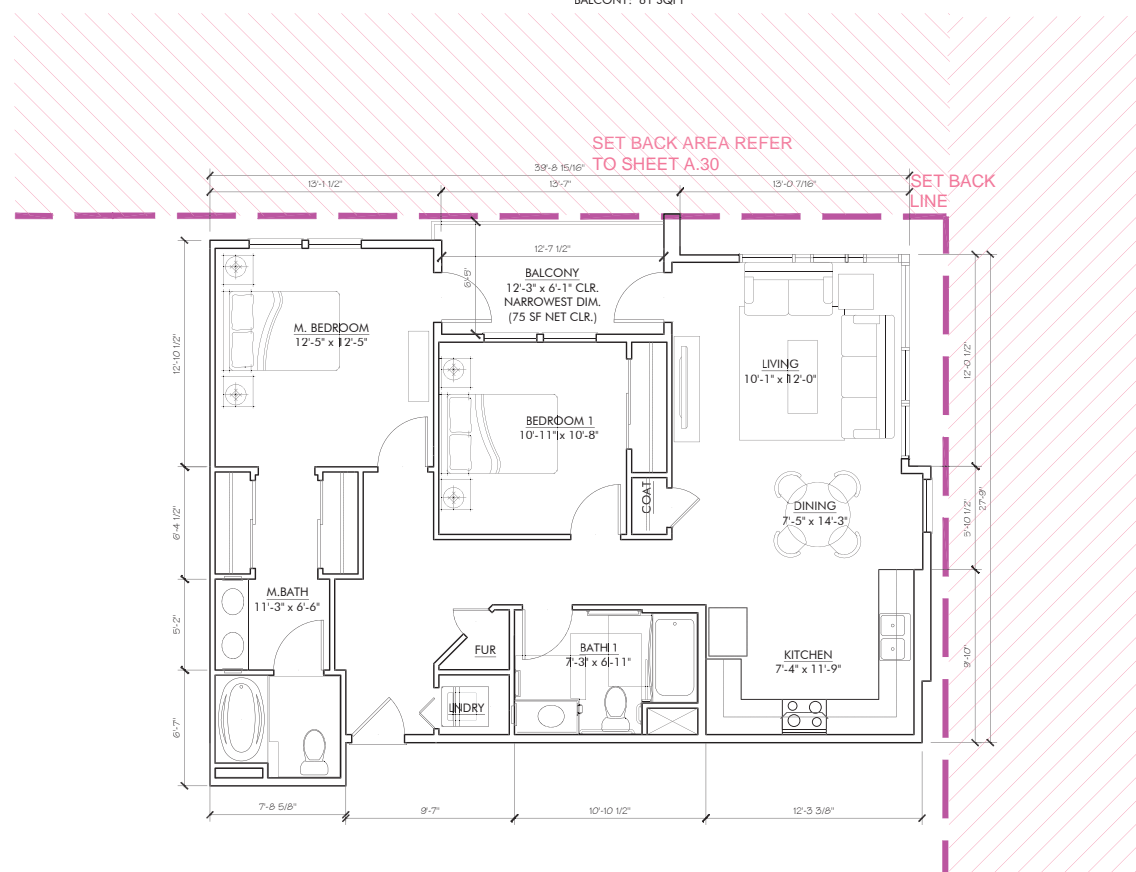
UNIT Q1 (CORNER) (2) BED UNIT PLAN GROSS AREA: 1,094 SQFT NET AREA: 1,009 SQFT BALCONY: 75 SQFT
