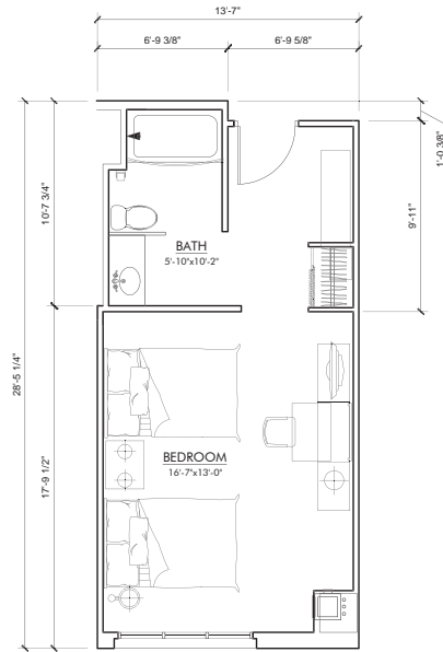
HOTEL ROOM A7 (2) BED UNIT FLOOR PLAN (Typ. 4th Floor Plan) GROSS AREA: 379 SQFT NET AREA: 332 SQFT
