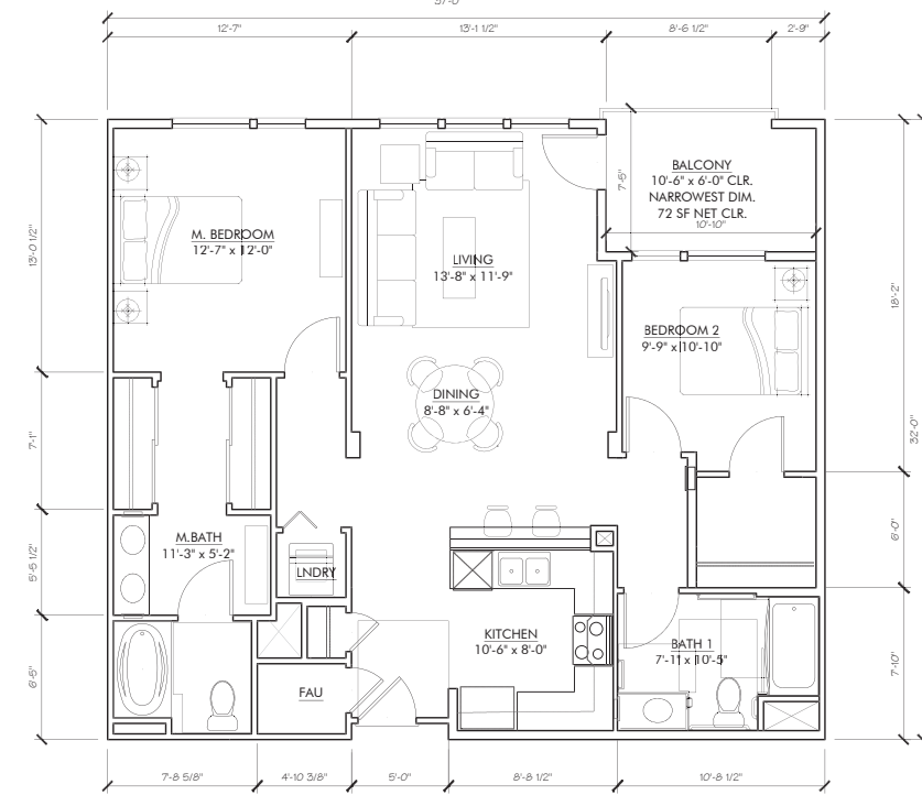
UNIT D1 (2) BED UNIT PLAN GROSS AREA: 1103 SQFT NET AREA: 1034 SQFT BALCONY: 72 SQFT
