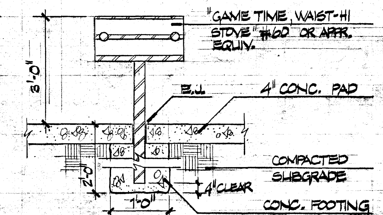
10 BARBEQUE L-4 1 st = 1-0
