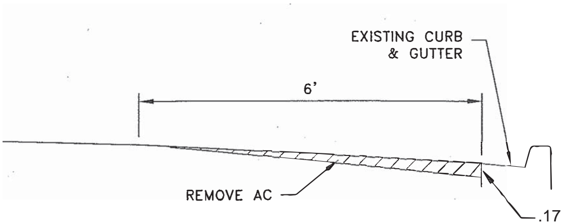
KEYCUT – TYPE A LONGITUDINAL KEYCUT NTS
