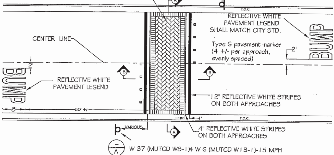
PLAN VIEW
