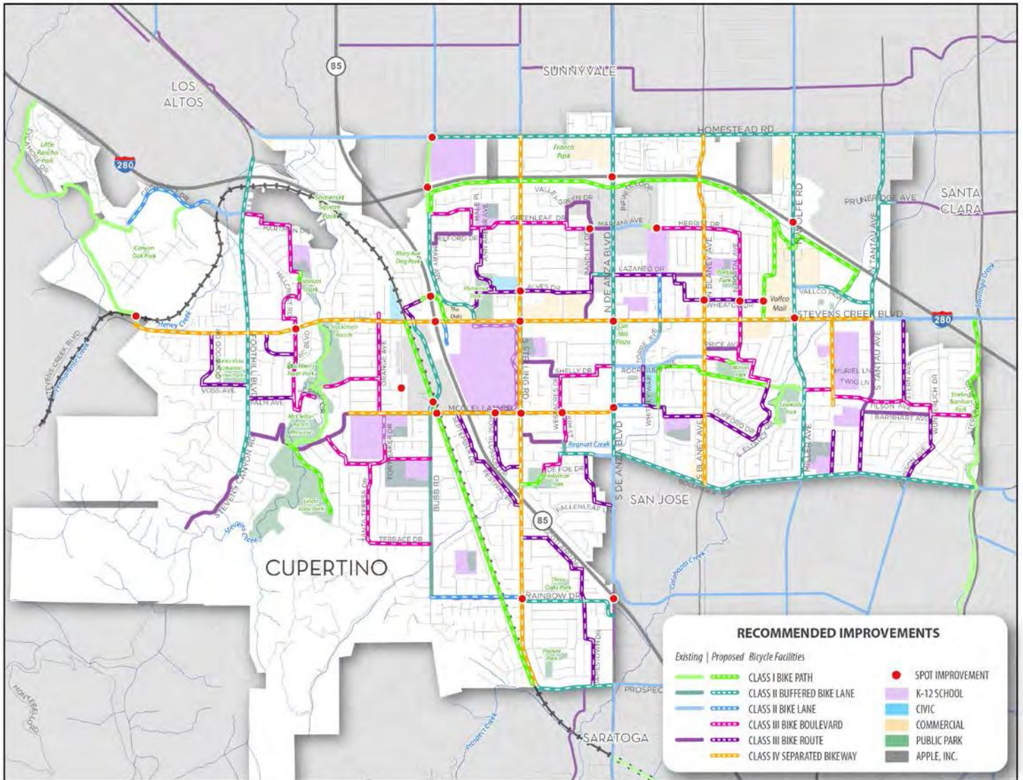
Figure 3-7: Bikeway projects
