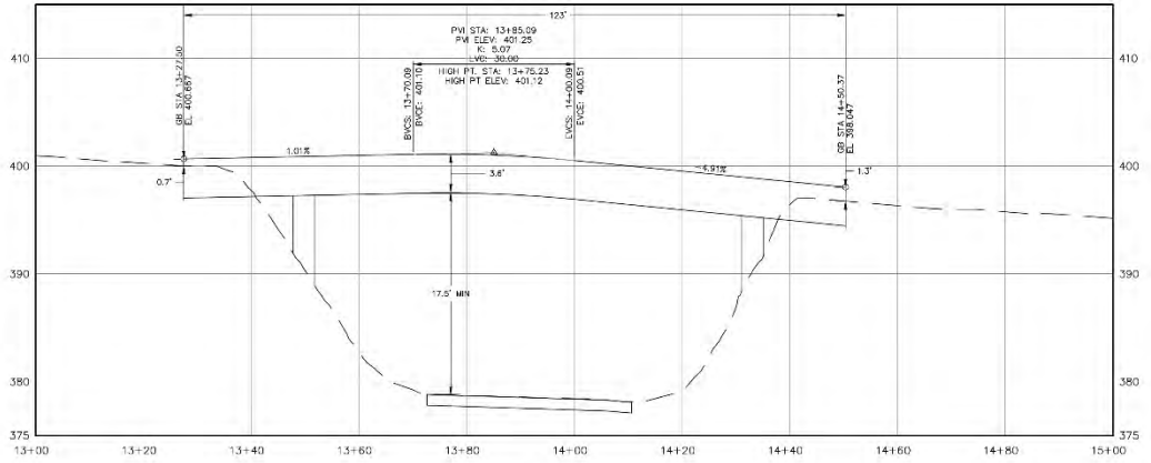
Profile Hr Scale: 1" = 10' Vt Scale: 1" = 8' Note: Foundation details not shown
