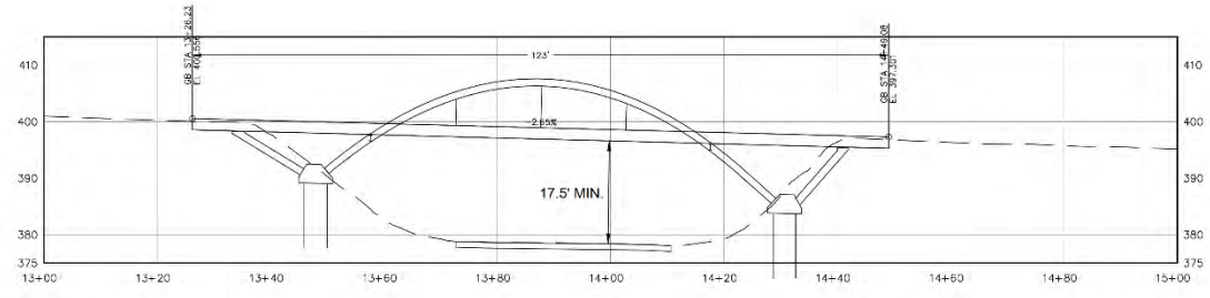
Profile Hz Scale: 1" = 10' Vt Scale: 1" = 10' Note: Foundation details not shown
