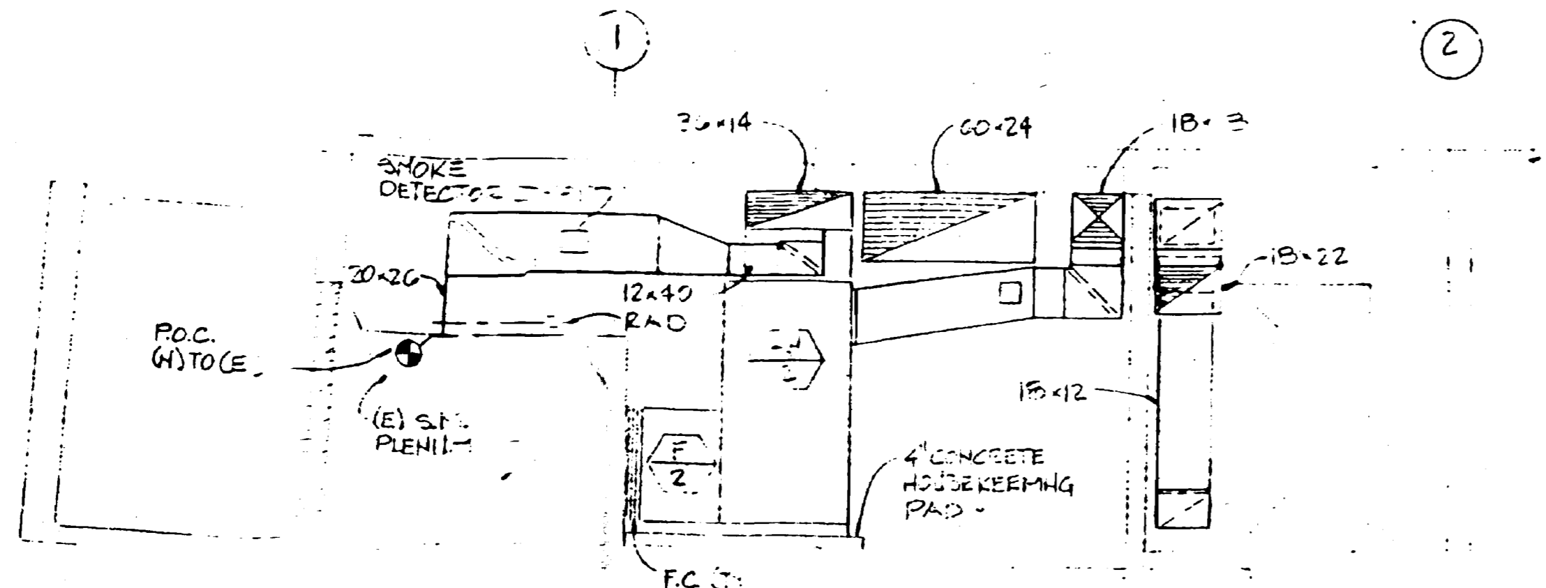
PARTIAL ROOF PLAN SCALE: 1/4" = 1'-0"
