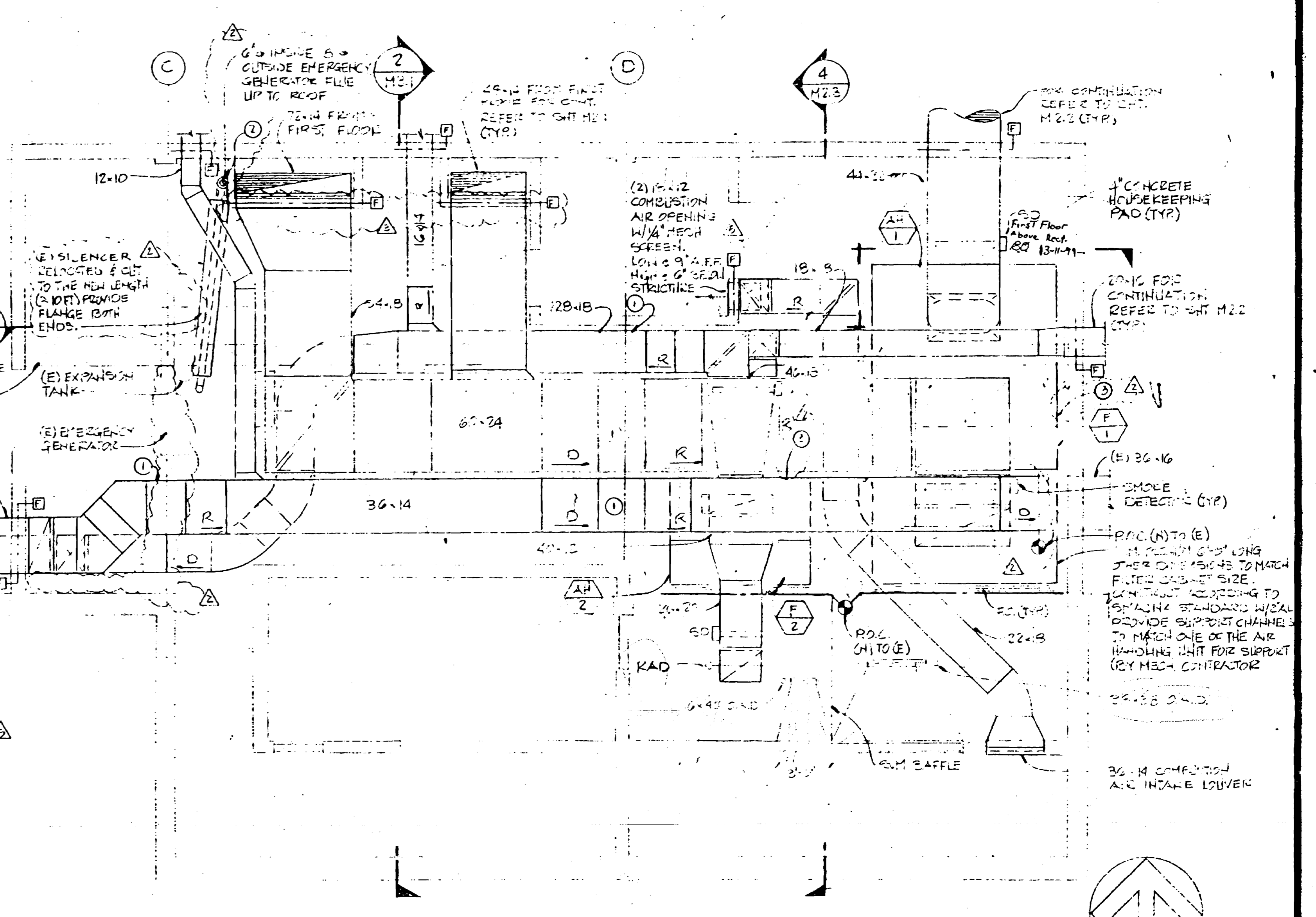
MECHANICAL RM PLAN SCALE: 1/4" = 1'-0"
