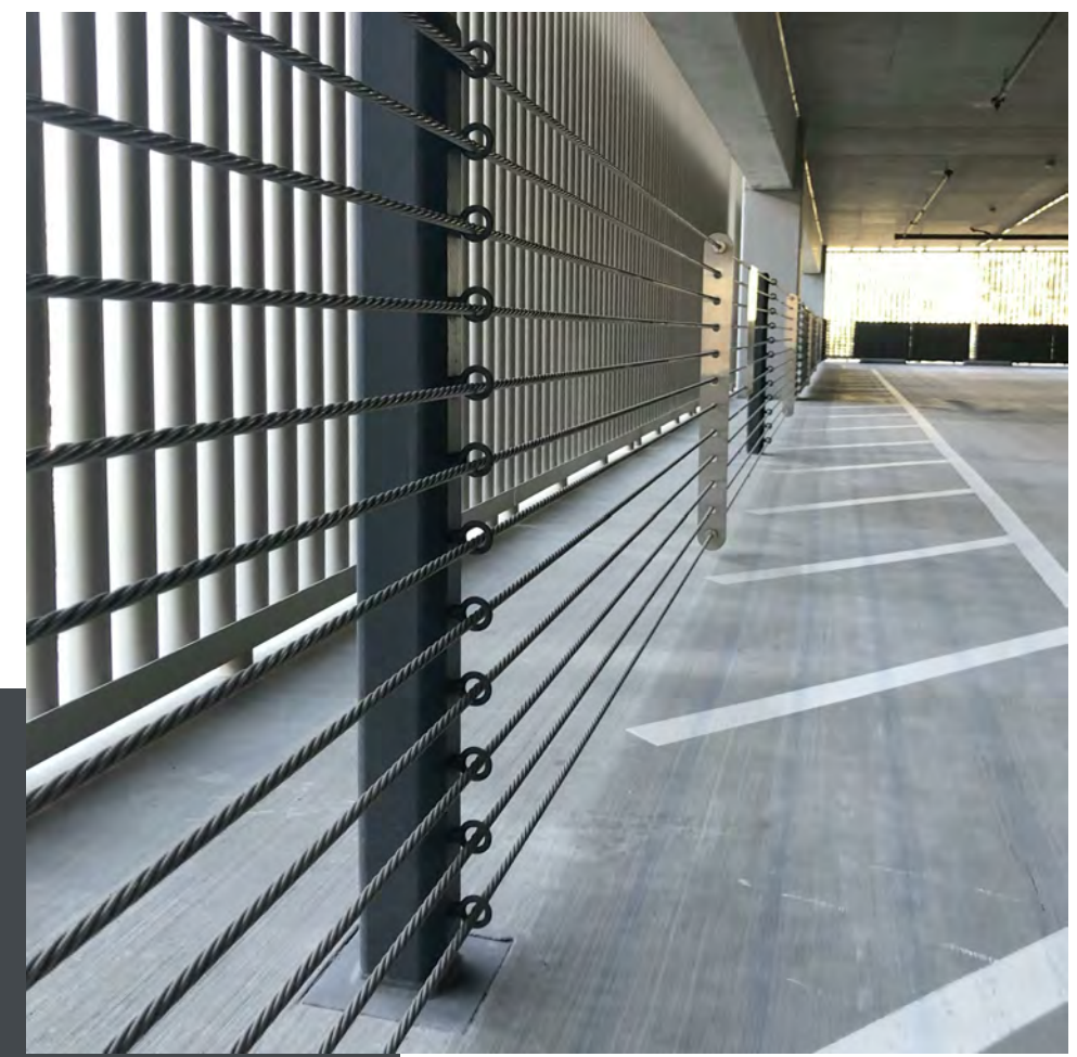
CABLE RAILING PARKING GARAGE GUARDRAIL (MTL4) TYPE: METAL PRODUCT: RAILING POST COLOR: RAL 7024 GRAPHITE GREY PROTECTED FINISH: PAINTED
